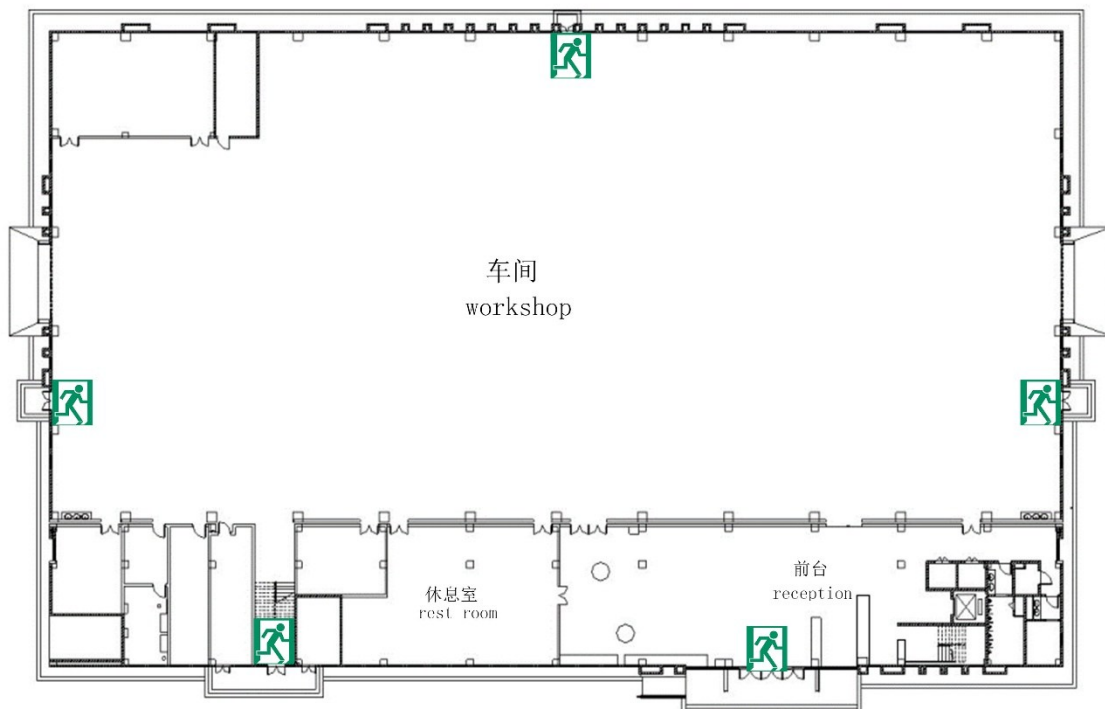
The Ground Floor of AEMTC
